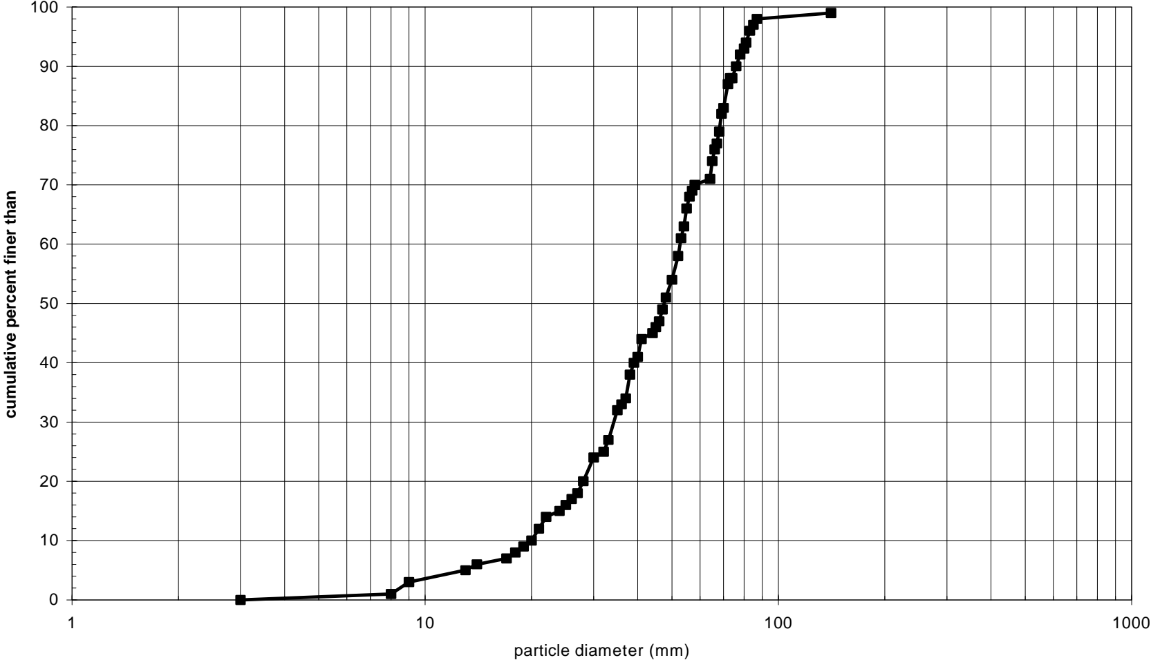
Figure C-1. Surface particle size distribution at Riffle 3
