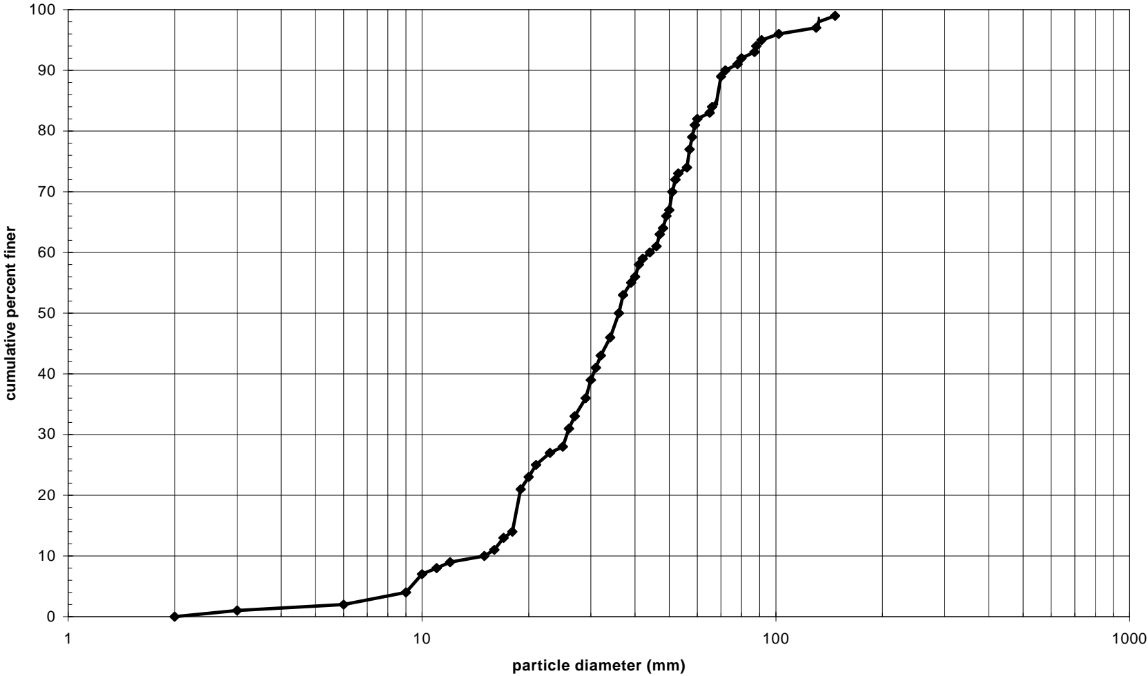
Figure C-6. Surface particle size distribution at Riffle 9b
