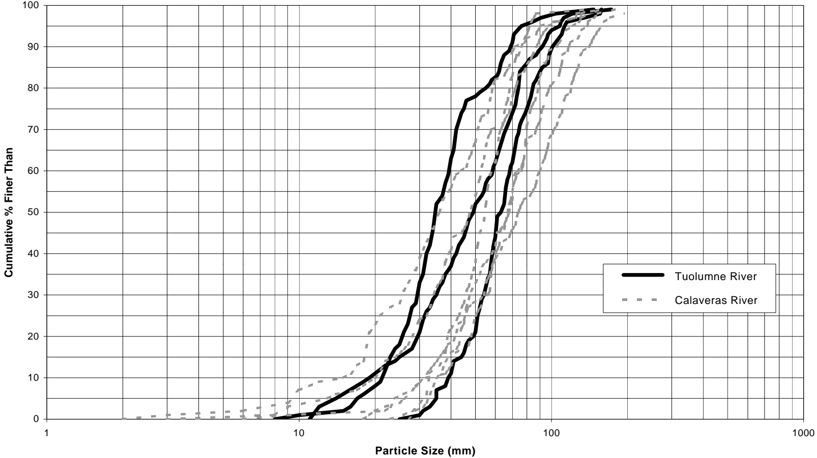
Figure C-7. Comparison of cumulative particle size distribution curves of spawning gravels used extensively by chinook salmon in the Tuolumne River, with potentially suitable spawning gravels in the Calaveras River
