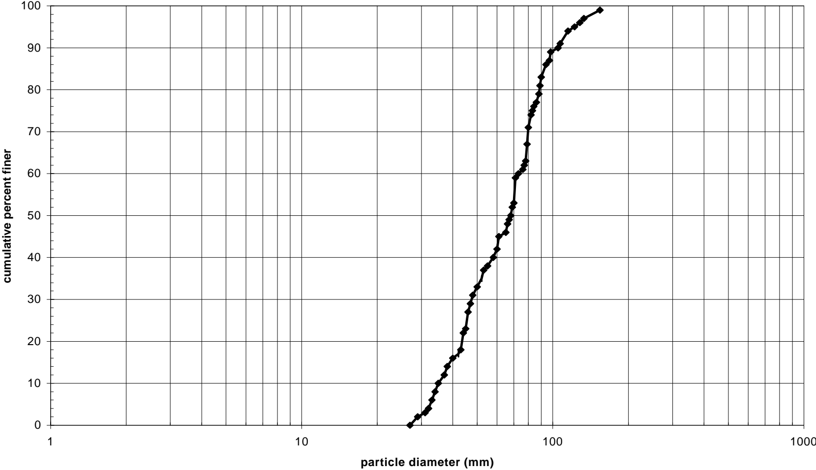
Figure C-3. Surface particle size distribution at Riffle 5
