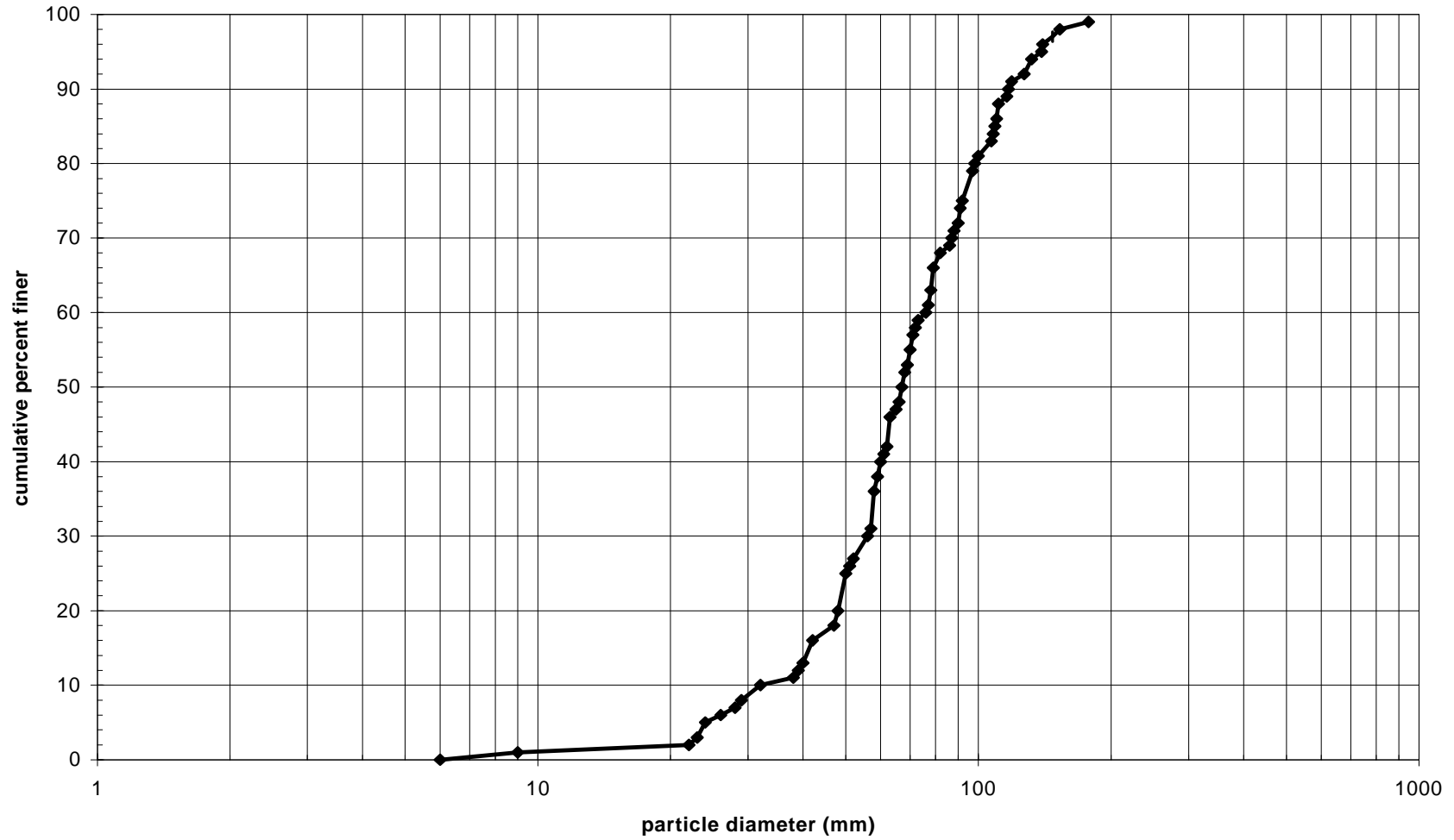
Figure C-2. Surface particle size distribution at Riffle 4
