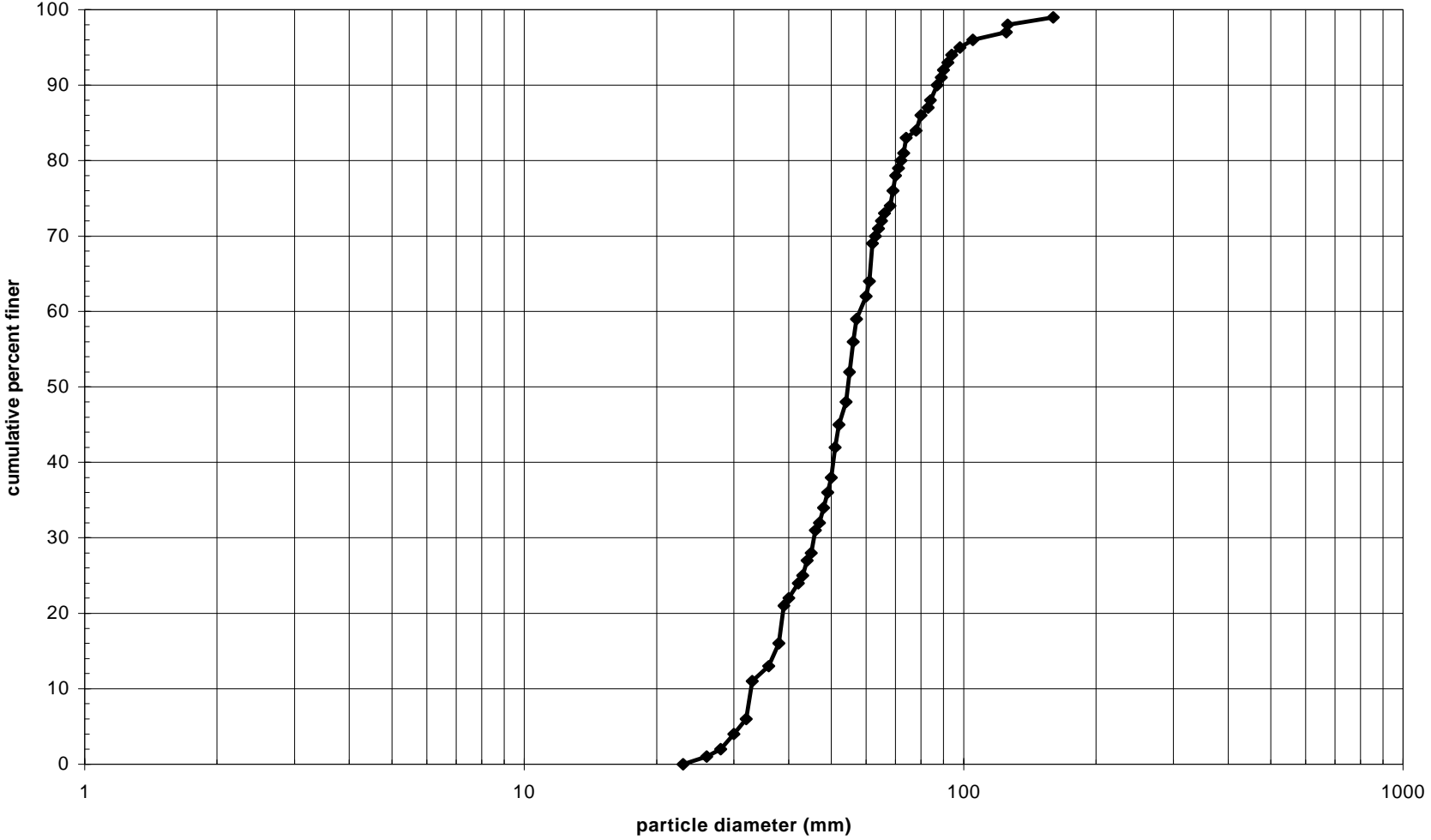
Figure C-5. Surface particle size distribution at Riffle 9a
