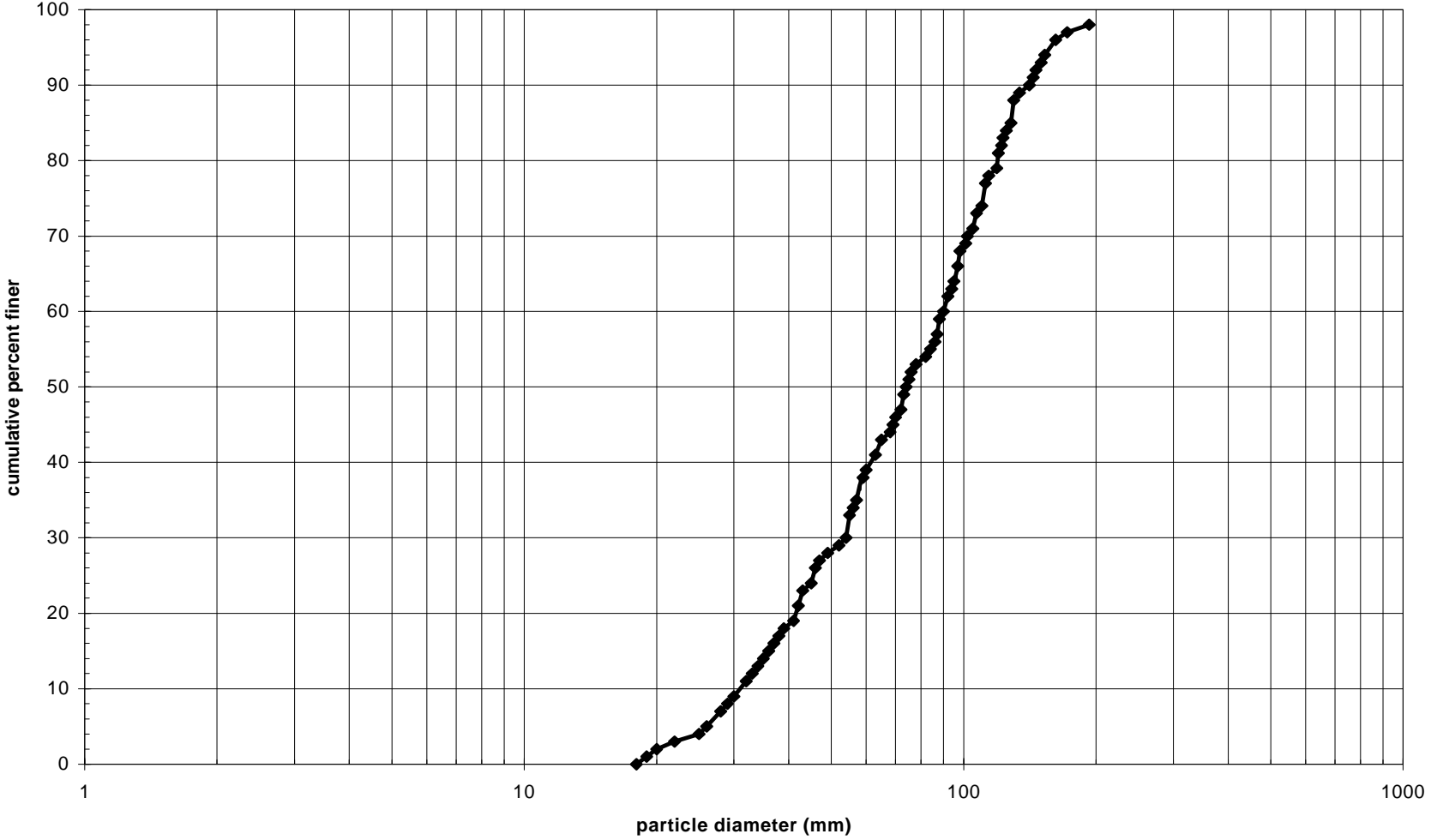
Figure C-4. Surface particle size distribution at Riffle 6
